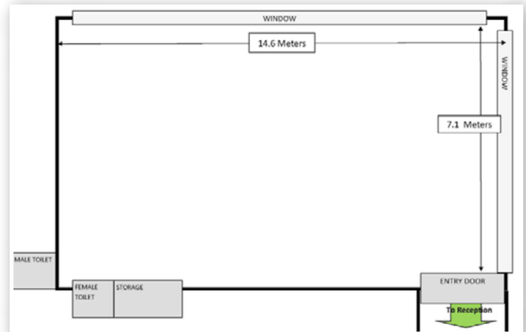
Wattle Room Floor Plan
